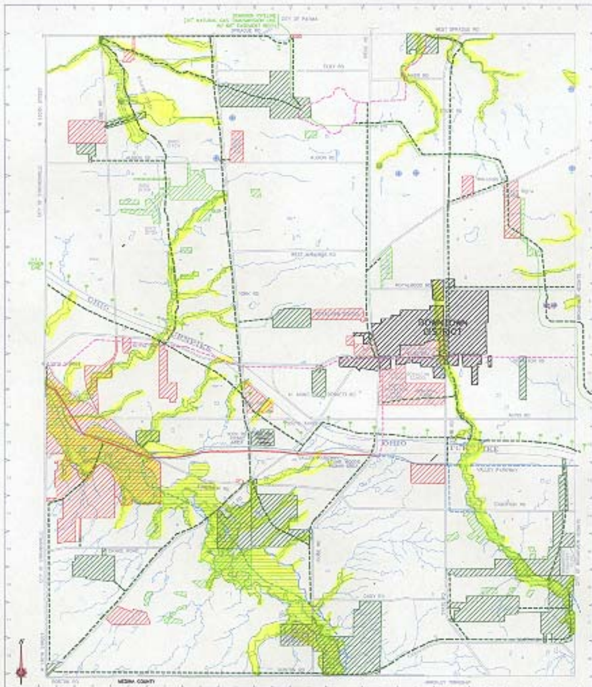
NORTH ROYALTON GREENWAYS PLAN CITY OF NORTH ROYALTON - OHIO SCALE IN FEET 0 100 200 300 400 500
